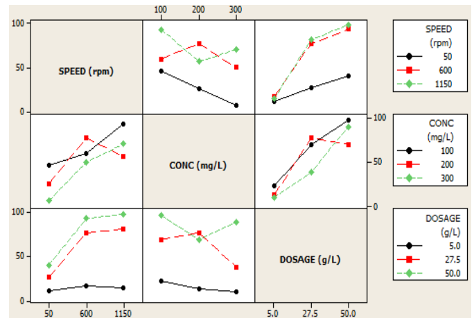
Fig. 2 Interaction plot for dye removal (%)
