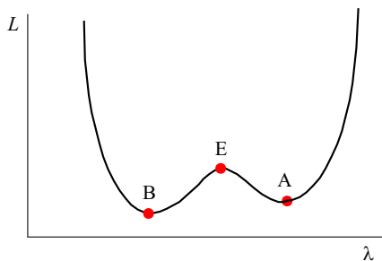
Fig. 5. Illustration of scalar cubic of (13) respect \lambda
