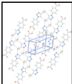
Fig. 2. A view of the supramolecular layer in (I) mediated by O—H...O, O—H...N and C—H...O interactions, shown as orange, blue and purple dashed lines, respectively.
