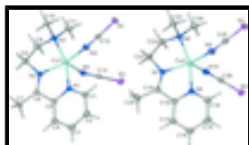
Fig. 1. The molecular structure of the title compound (50% probability ellipsoids). Hydrogen atoms are drawn as spheres of arbitrary radius.
