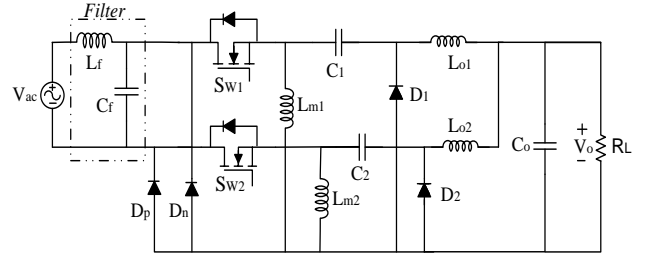
Fig. 2. Proposed bridgeless Zeta PFC.
