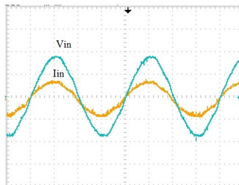
Fig. 12. Line voltage and input line current [V: 100V/div, I: 1 A/div, t: 5 ms/div].
