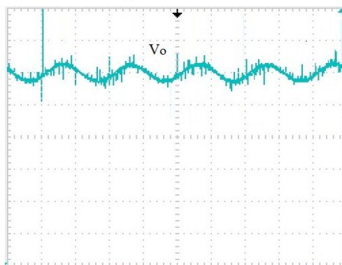
Fig. 13. Output voltage ripple at 60V dc [V: 5V/div, t: 10 ms/div].
