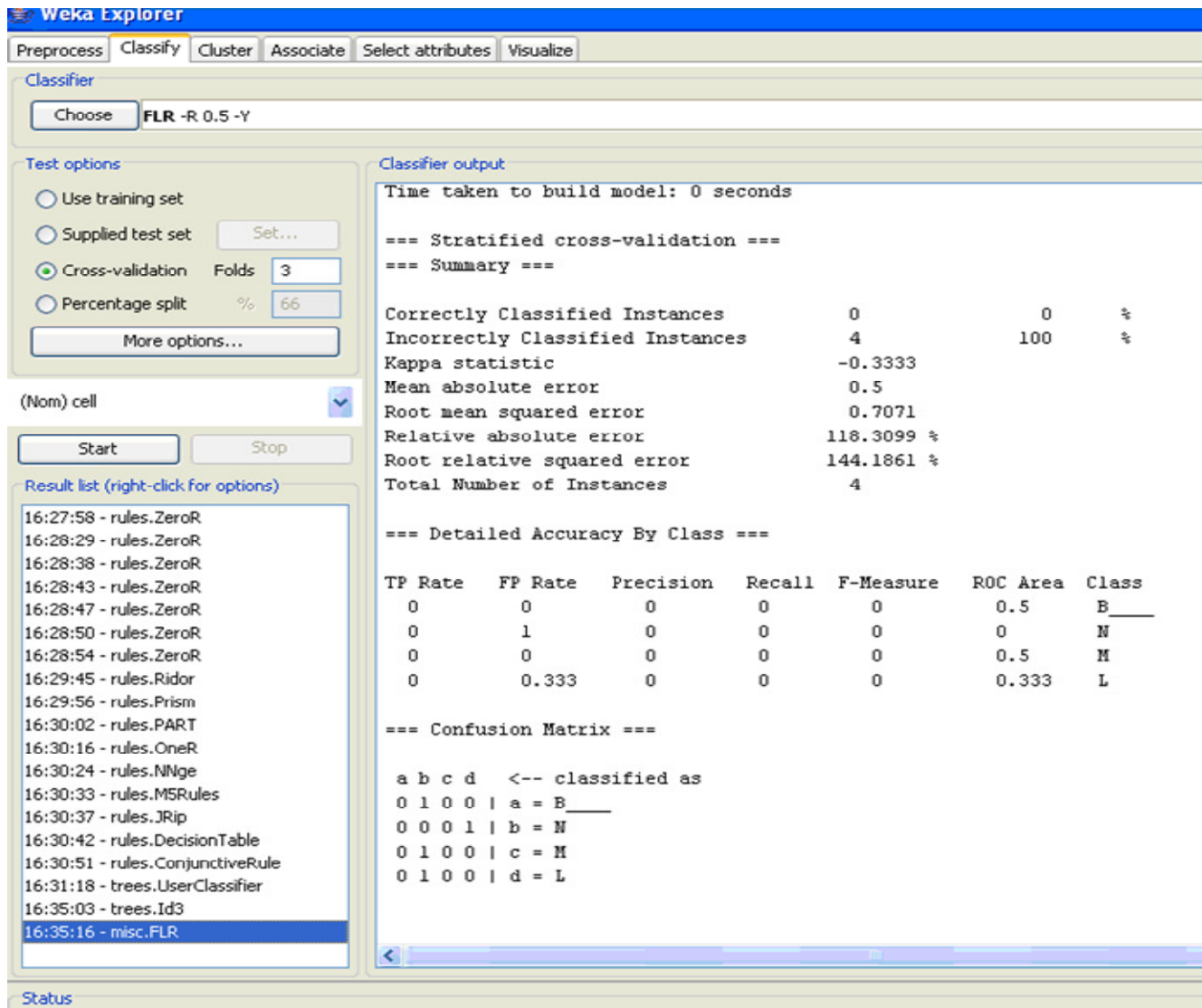
Figure 6. Classification of individual cells. Courtesy :Weka.
