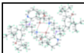
Fig. 1. Thermal ellipsoid plot (Barbour, 2001) of O—H...O hydrogen-bonded dimeric structure of [(C 4 H 9 ) 2 NH 2 ] [C 21 H 26 NO 3 S] at the 70% probability level. Dashed lines denote the intra-ionic hydrogen bonds in the salt. Hydrogen atoms are drawn as spheres of arbitrary radius.
