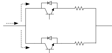
Figure 5: Circulating Current during One Switching Cycle
