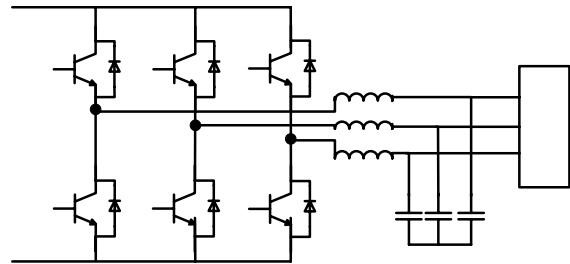
Figure 1: Three-Phase Inverter
