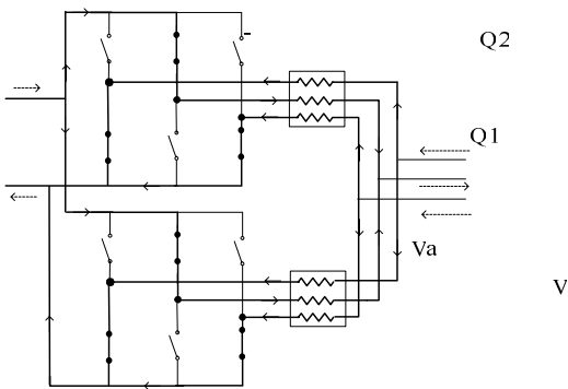
Figure 10: The current path during Mode 4.
