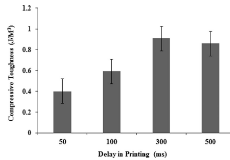
Fig. 8. Comparison of compressive toughness in samples printed with different layer printing delays.
