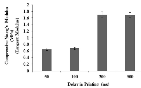
Fig. 7. Comparison of compressive tangent modulus in samples printed with different layer printing delays.
