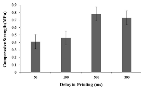
Fig. 6. Comparison of compressive strength in samples printed with different layer printing delays.
