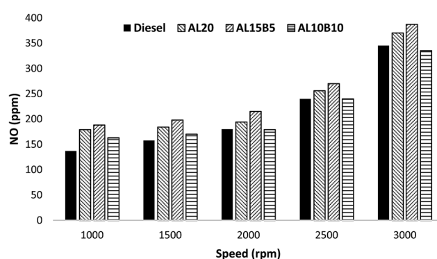
Fig. 7 NO emission vs. speed diagram for AL biodiesel and its modified blends at 80 Nm torque.
