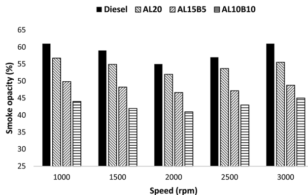
Fig. 10 Smoke opacity vs. speed diagram for AL biodiesel and its modified blends at 80 Nm torque.
