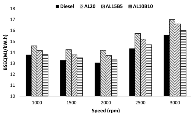
Fig. 5 BSEC vs. speed diagram for AL biodiesel and its modified blends at 80 Nm torque.
