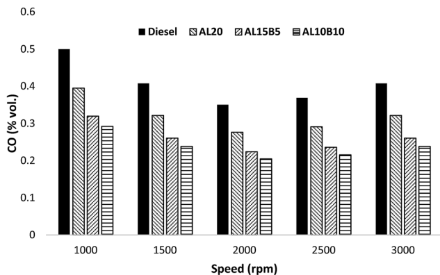
Fig. 8 CO emission vs. speed diagram for AL biodiesel and its modified blends at 80 Nm torque.
