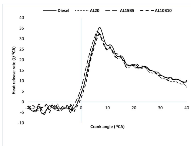
Fig. 3 Heat release rate vs. crank angle diagram for n -butanol blends at 2000 rpm.
