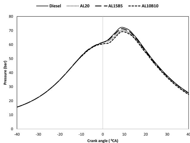
Fig. 2 Cylinder pressure vs. crank angle diagram for n -butanol blends at 2000 rpm.
