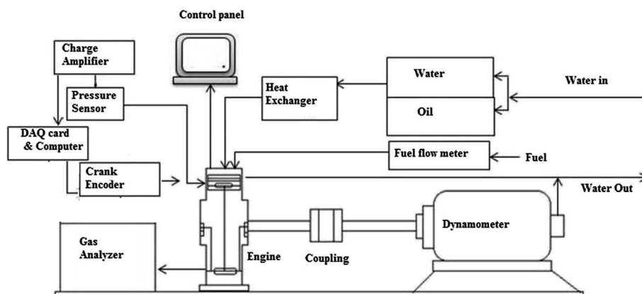
Fig. 1 Schematic diagram of the engine test bed.
