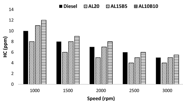
Fig. 9 HC emission vs. speed diagram for AL biodiesel and its modified blends at 80 Nm torque.
