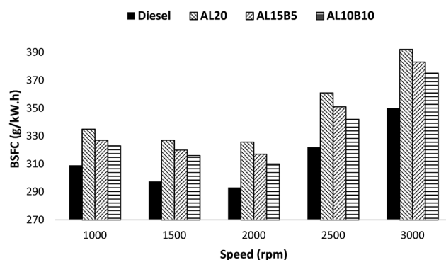
Fig. 4 BSFC vs. speed diagram for AL biodiesel and its modified blends at 80 Nm torque.
