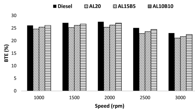
Fig. 6 BTE vs. speed diagram for AL biodiesel and its modified blends at 80 Nm torque.
