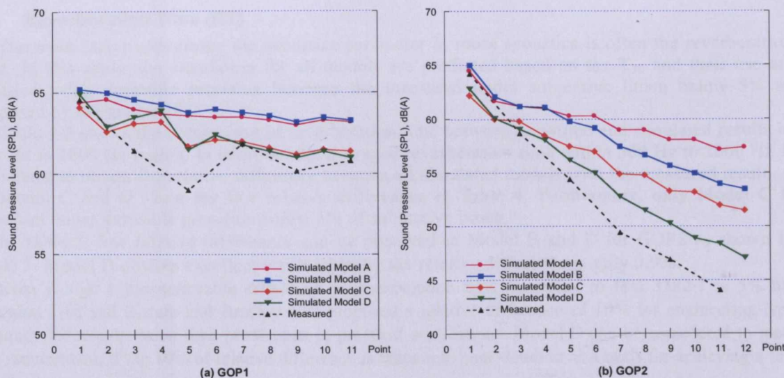
Figure 5 – Comparison of sound pressure level between measured and models simulated.
