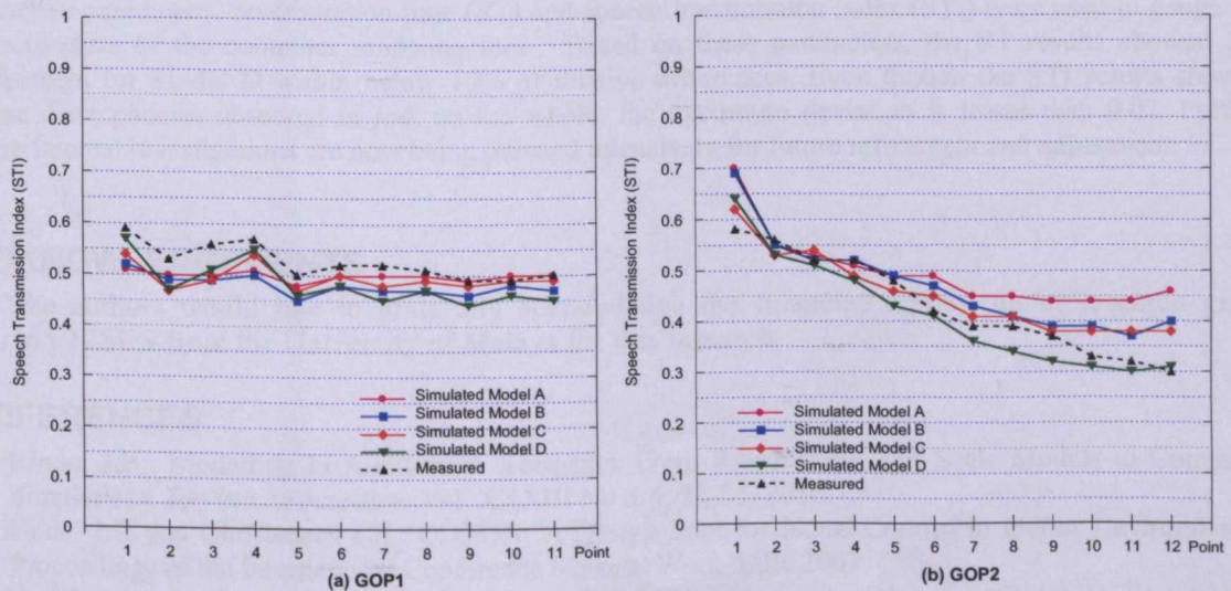
Figure 6 – Comparison of speech transmission index (STI) between measured and models simulated.
