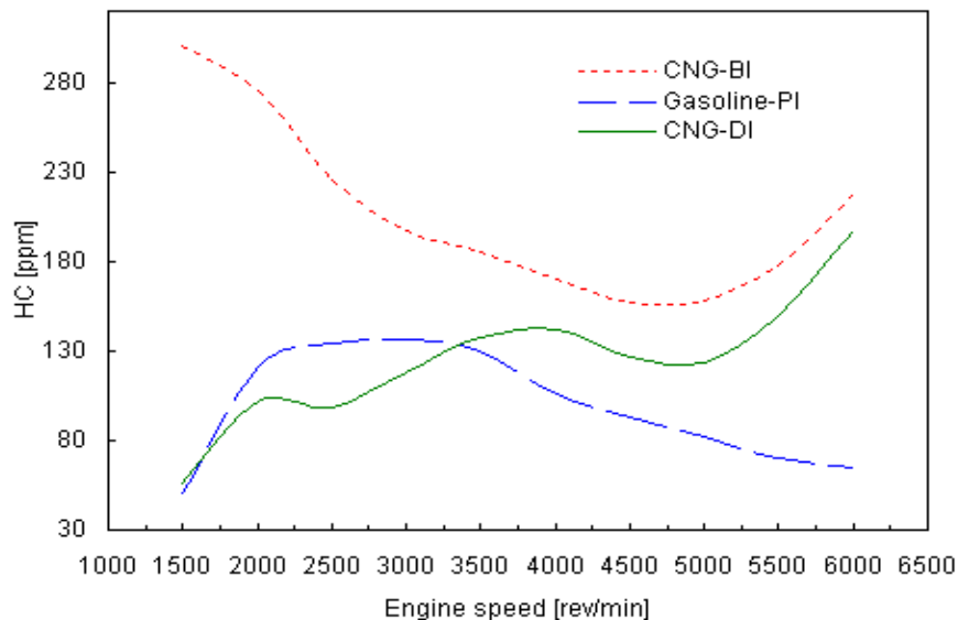
Figure 6: Unburned Hydrocarbon Versus Engine Speed at WOT.
