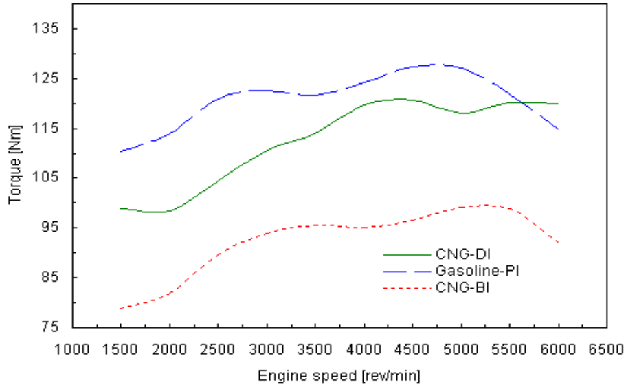
Figure 4: Brake Torque Versus Engine Speed at WOT
