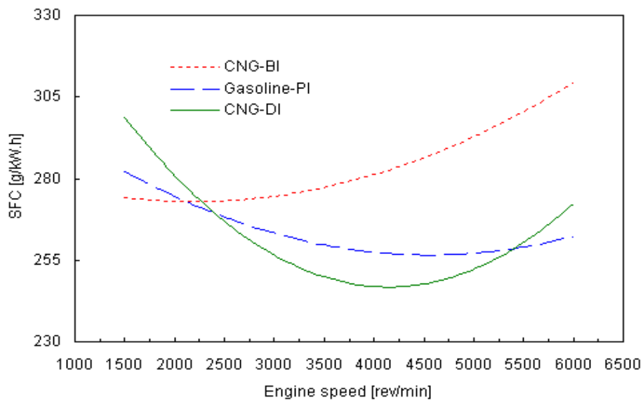
Figure 5: Brake Specific Fuel Consumption Versus Engine Speed at WOT
