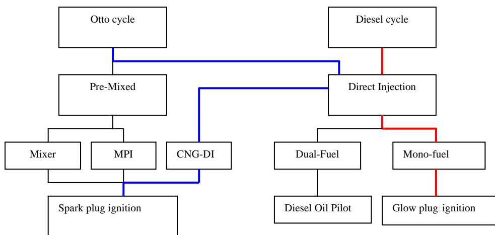
Figure 1: Various Combustion Systems for CNG Fuel
