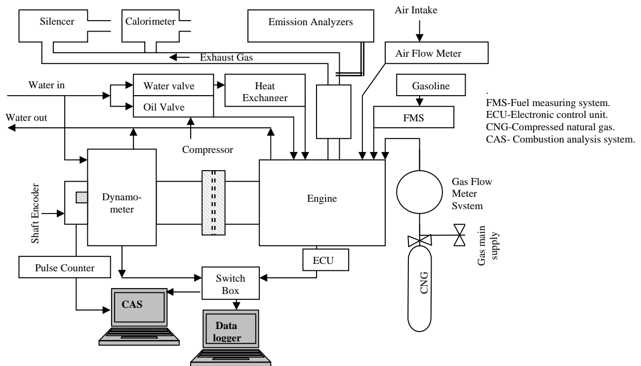
Figure 2: Schematic Diagram of the Experimental Set-Up
