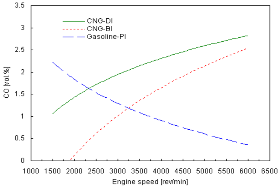
Figure 8: Carbon Monoxide Versus Engine Speed at WOT
