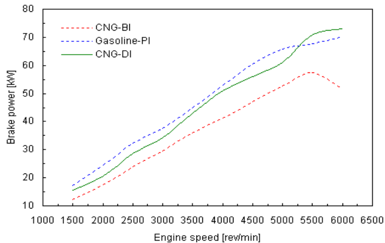
Figure 3: Brake Power Versus Engine Speed at WOT
